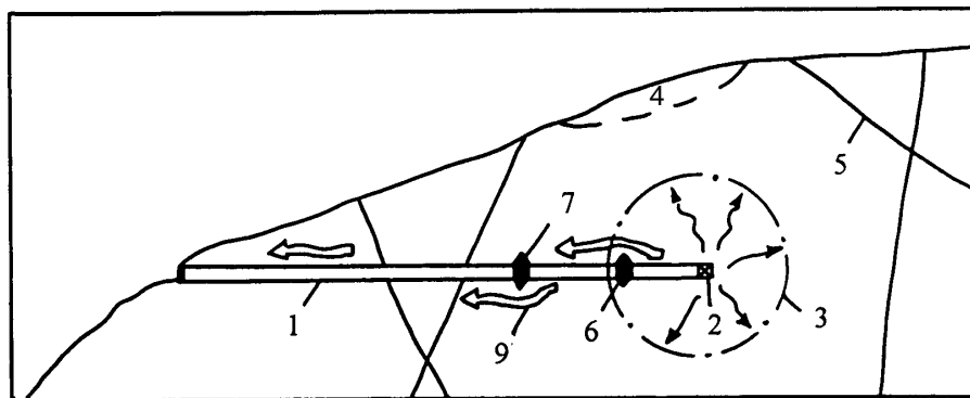
Figure 21. Illustration of gas release through the tunnel by migration around the stemming plugs: 1- tunnel works; 2- zero room; 3- damage zone radius; 4- spill zone; 5- tectonic faults; 6 and 7- first and second stemming; 9- gas flow through the tunnel and surrounding rock.
